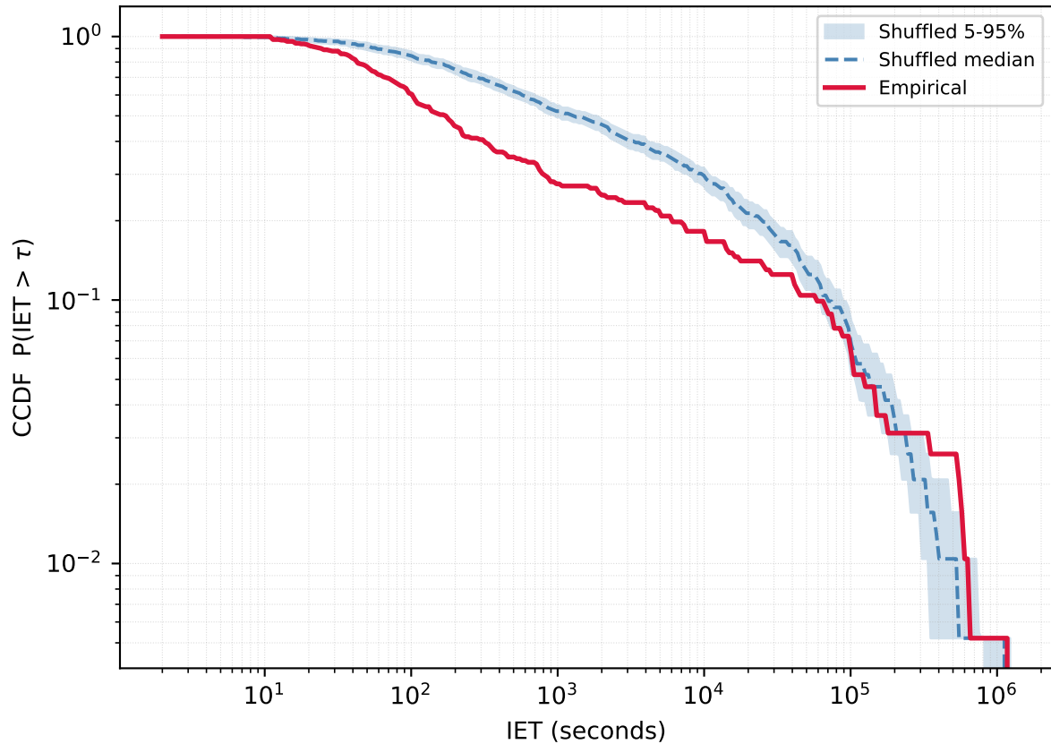
User 698141415 - Empirical vs Reshuffled | KS=0.312 p=0.000
