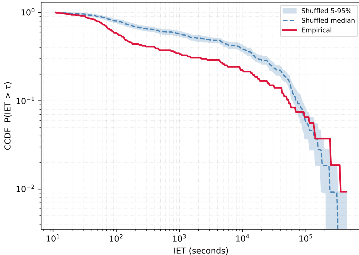
User 675391573 - Empirical vs Reshuffled | KS=0.273 p=0.000
