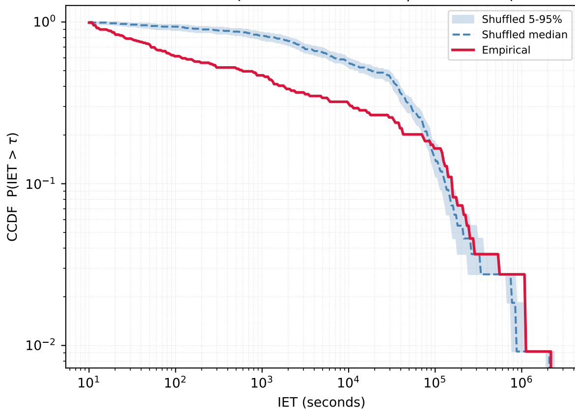
User 882741473 - Empirical vs Reshuffled | KS=0.394 p=0.000
