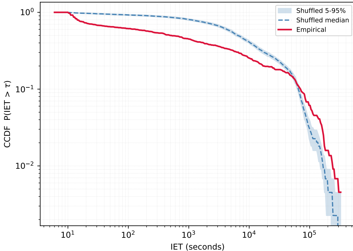
User 323309626 - Empirical vs Reshuffled | KS=0.373 p=0.000
