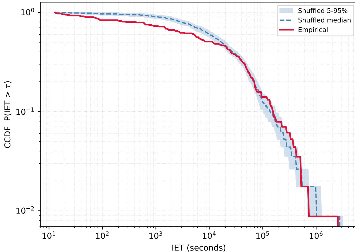
User 405690380 - Empirical vs Reshuffled | KS=0.204 p=0.000
