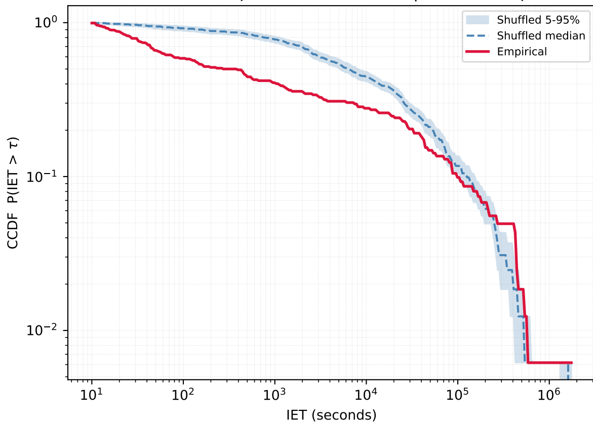
User 36162471 - Empirical vs Reshuffled | KS=0.405 p=0.000
