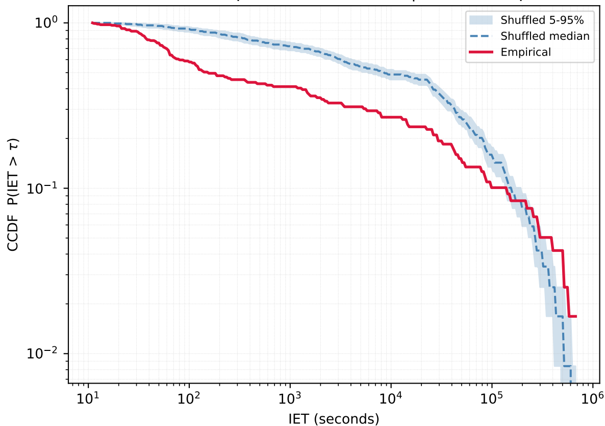
User 5357949 - Empirical vs Reshuffled | KS=0.391 p=0.000
