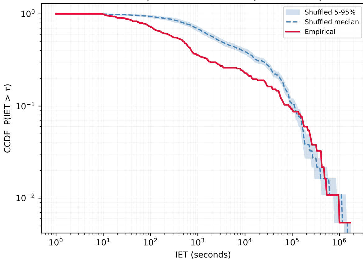
User 17798588 - Empirical vs Reshuffled | KS=0.363 p=0.000
