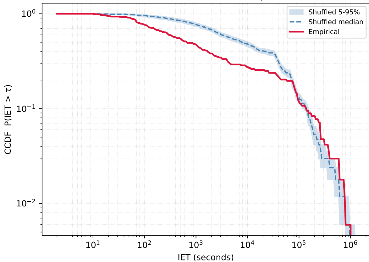
User 185880661 - Empirical vs Reshuffled | KS=0.330 p=0.000
