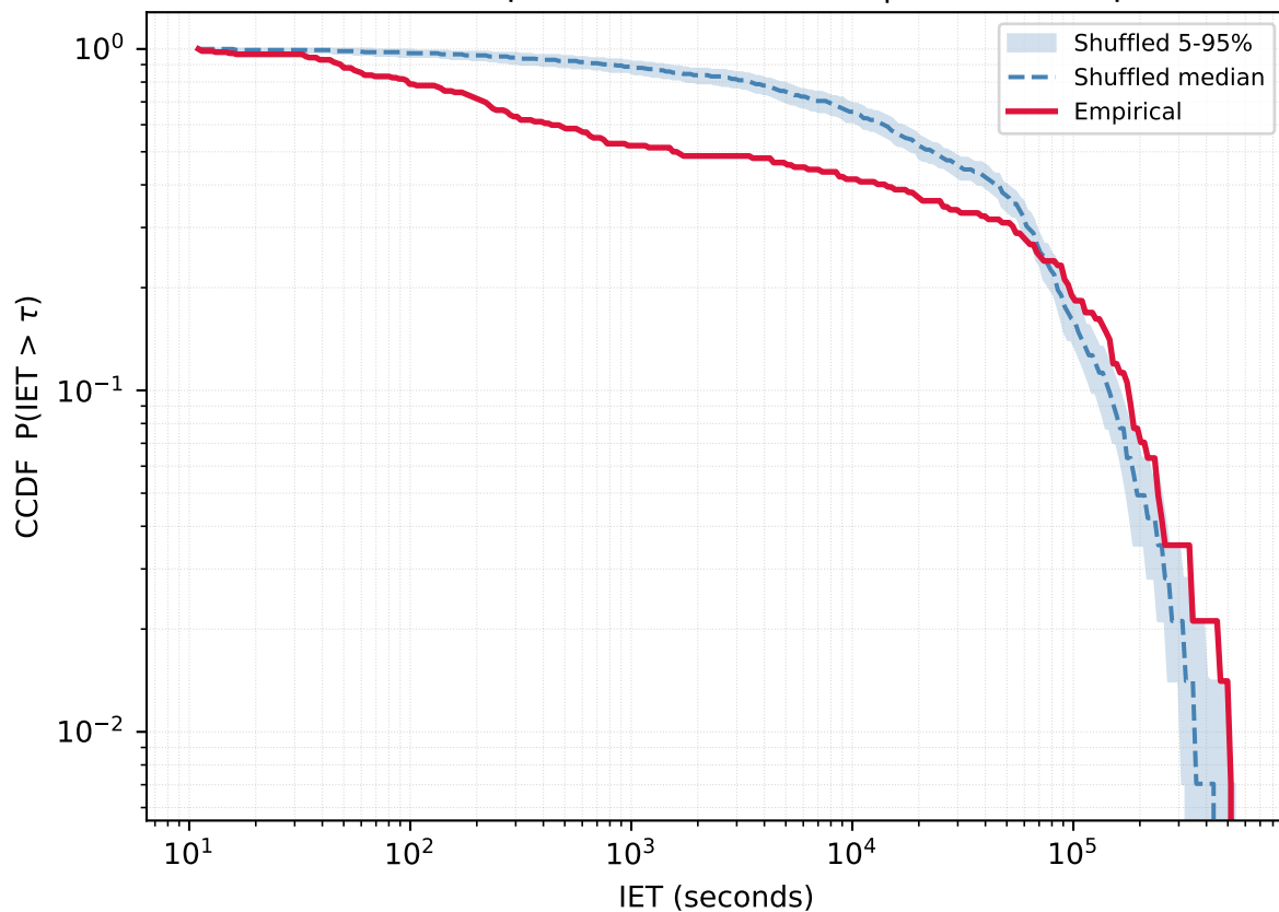
User 7678561 - Empirical vs Reshuffled | KS=0.376 p=0.000
