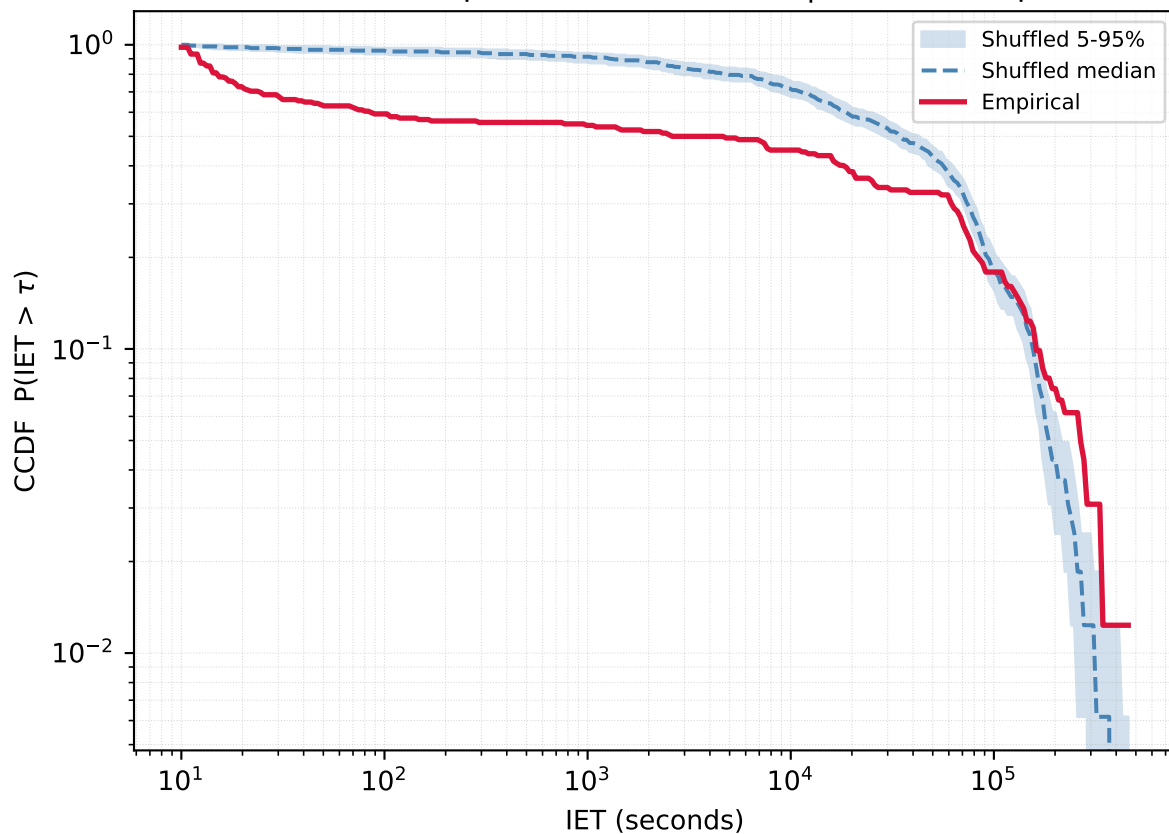
User 4473225 - Empirical vs Reshuffled | KS=0.389 p=0.000
