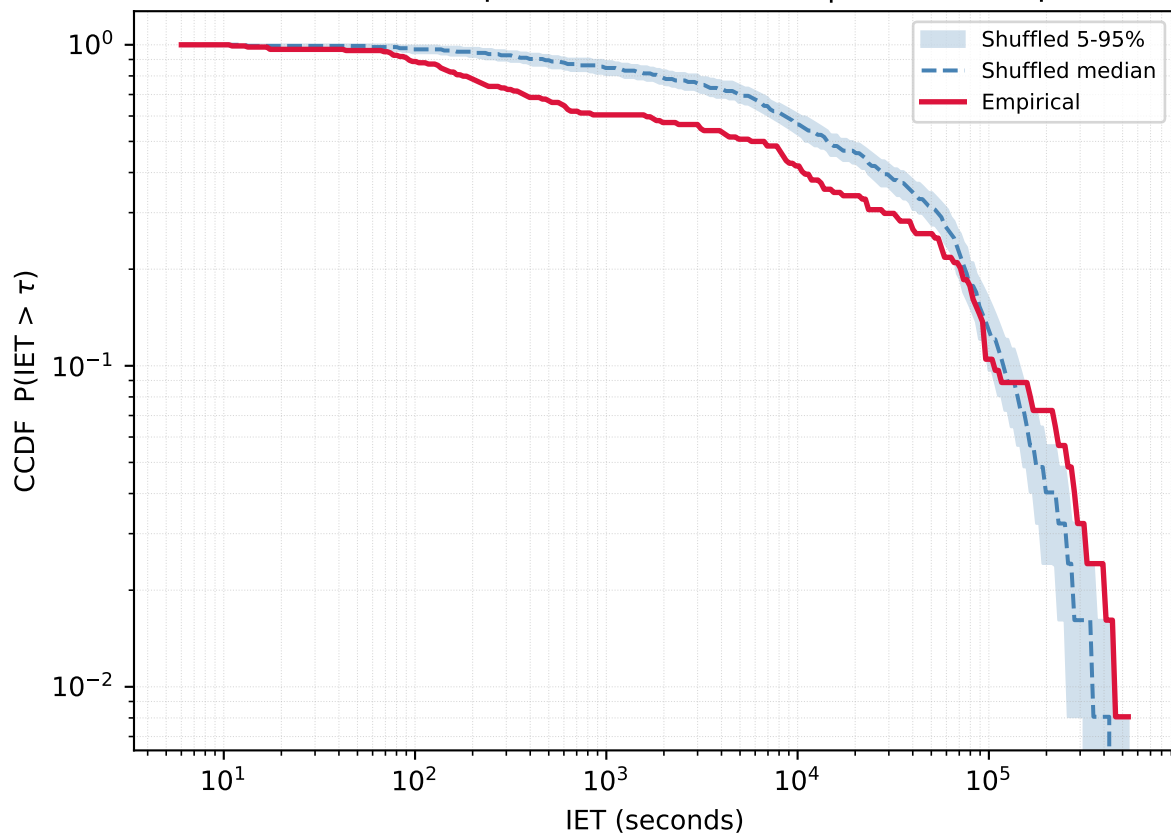
User 458678536 - Empirical vs Reshuffled | KS=0.258 p=0.000
