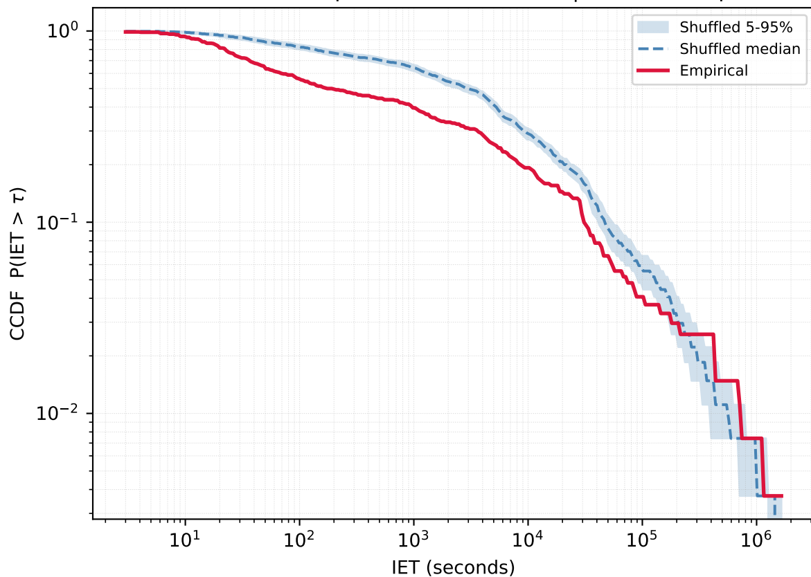
User 145800528 - Empirical vs Reshuffled | KS=0.284 p=0.000
