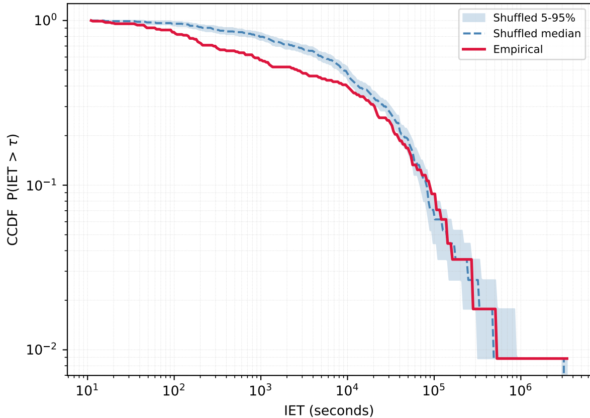
User 459294324 - Empirical vs Reshuffled | KS=0.244 p=0.000
