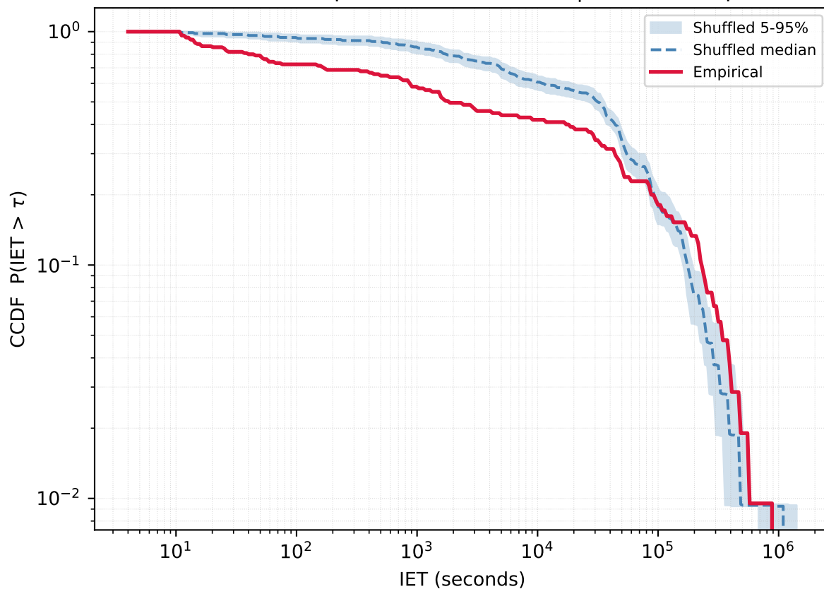
User 78947024 - Empirical vs Reshuffled | KS=0.307 p=0.000
